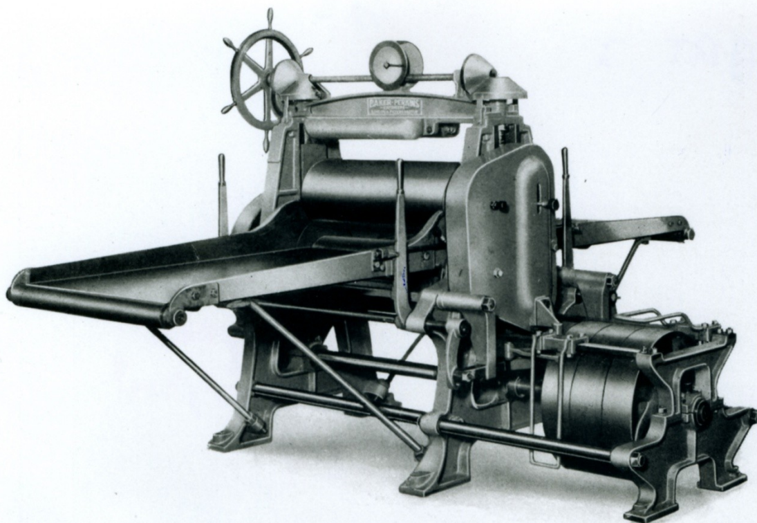
"Baker-Thomson" Power Reversing Hard and Soft Dough Brake
