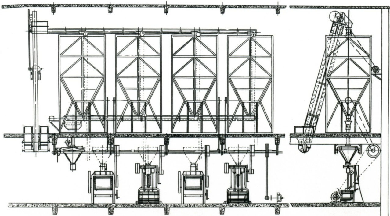
FLOUR HANDLING PLANT with STORAGE HOPPERS
