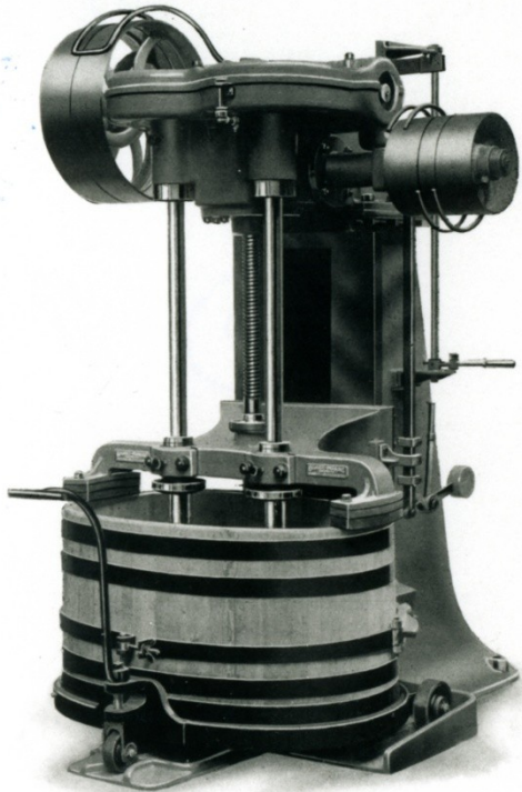
“ Baker-Thomson ” Vertical Mixing Machine
