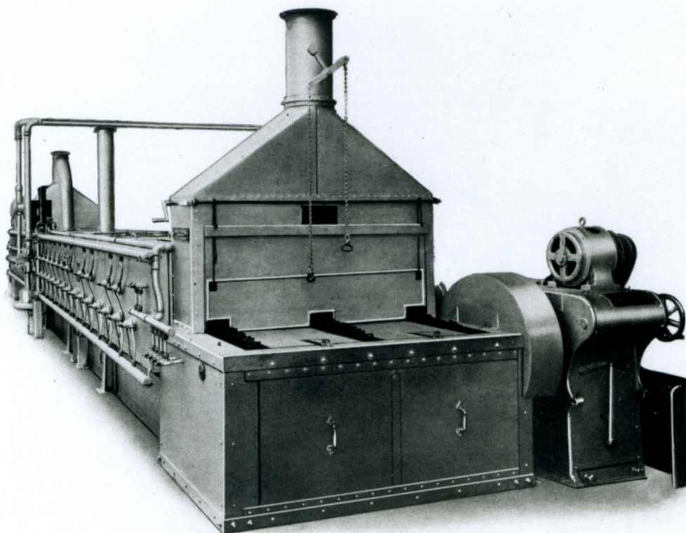
Delivery End of "Baker-Keith" Patent Gas-Fired Travelling Chain Oven showing combined driving gear and latest type pre-mixing Gas equipment
